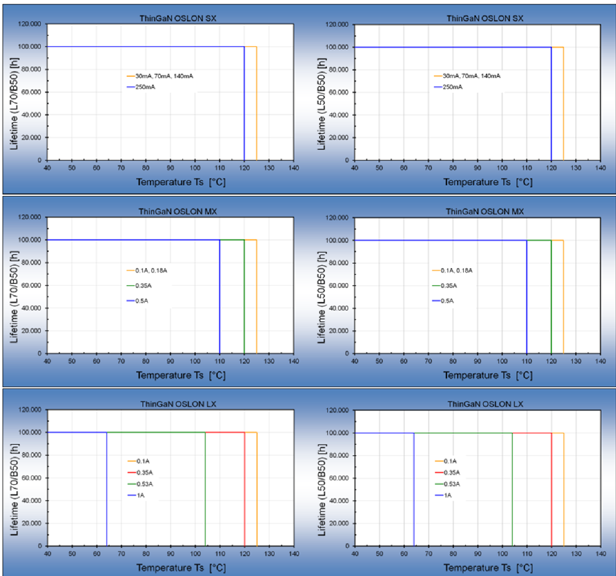
Figure 5a: Lifetimes (*) of the OSLOM types (SX, MX, LX) with ThinGaN technology with respect to T_s
