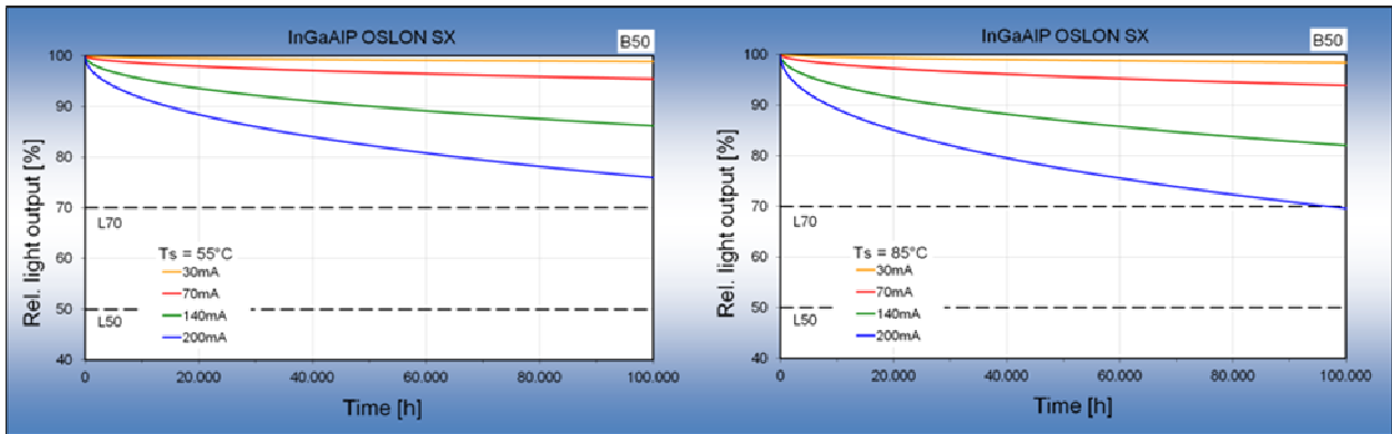
Figure 8: Degradation characteristics (*) of the OSLOX SX with ThinFilm technology for T_s=55^\circ\text{C} & T_s= 85^\circ\text{C} (grouping current I_F = 0,14\text{A} )
