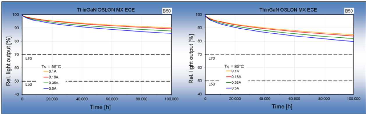
Figure 6: Degradation characteristics (*) of the OSLOM MX ECE (LxW CN7N) for T_S=55^\circ\text{C} & T_S= 85^\circ\text{C} (grouping current I_F = 0,35\text{A} )
