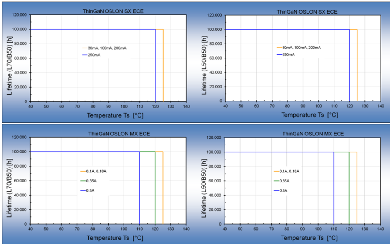
Figure 5b: Lifetimes (*) of the OSLON types (SX ECE, MX ECE) with ThinGaN technology with respect to T_S
