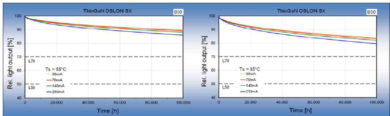
Figure 6a: Degradation characteristics (*) of the OSLON SX (Lx CN5M) for T_S=55\text{ °C} & T_S=85\text{ °C} (grouping current I_F = 0,14\text{ A} )
