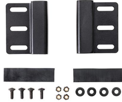
LGMT-001A Air Case Roof Mount
