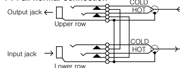
Full Normal Format (series)
