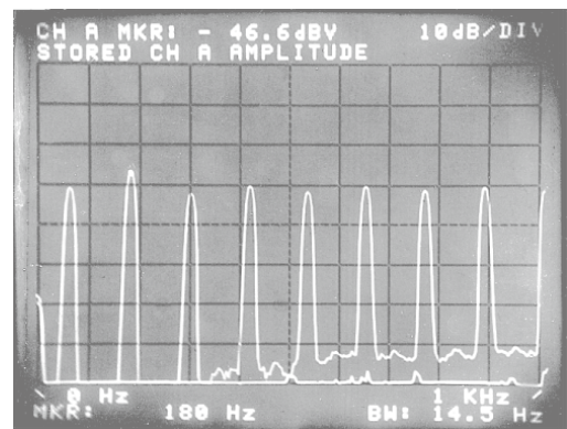
Fig. 1 Noise induced in two-conductor shielded cable (MVVS)
