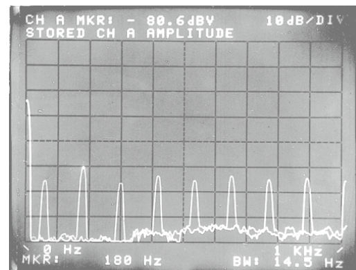
Fig. 2 Noise induced in star quad cable (Canare L-4E5AT)
