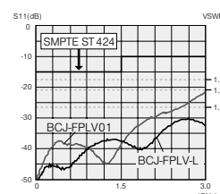
Return loss for BCJ-FPLV-L
