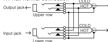
Half Normal Format (half-parallel)
