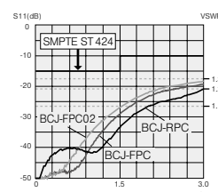
Return loss for BCJ-FPC, BCJ-FPC02, BCJ-RPC
