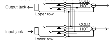
Double Normal Format (series-parallel)
